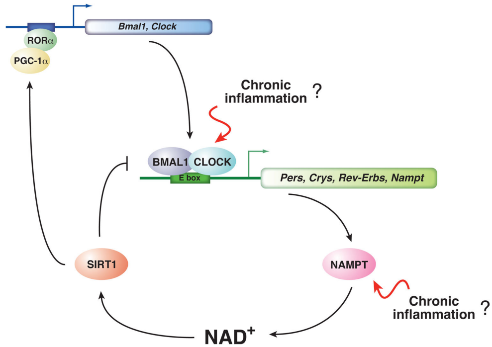
Figure 3. Synthesis of \text{NAD}^+ is regulated by the circadian clock and declines with age. The oscillating clock consists of the heterodimeric complex of core circadian transcription factors BMAL1 and CLOCK. The BMAL1/CLOCK complex controls the Nampt gene encoding the key \text{NAD}^+ biosynthetic enzyme nicotinamide phosphoribosyltransferase (NAMPT), rendering \text{NAD}^+ production and SIRT1 activity circadian in peripheral tissues. SIRT1 negatively regulates the transcriptional activity of the BMAL1/CLOCK complex, completing a novel circadian-regulatory feedback loop. In the suprachiasmatic nucleus (SCN), SIRT1 also regulates Bmal1 and Clock expression levels via the complex with PGC-1 \alpha and ROR \alpha . Chronic inflammation, particularly induced by inflammatory cytokines such as TNF- \alpha , might affect NAMPT-mediated \text{NAD}^+ biosynthesis and BMAL1/CLOCK-mediated circadian transcription in peripheral tissues and the SCN, causing a decline in the amplitude of the circadian clock with age.
