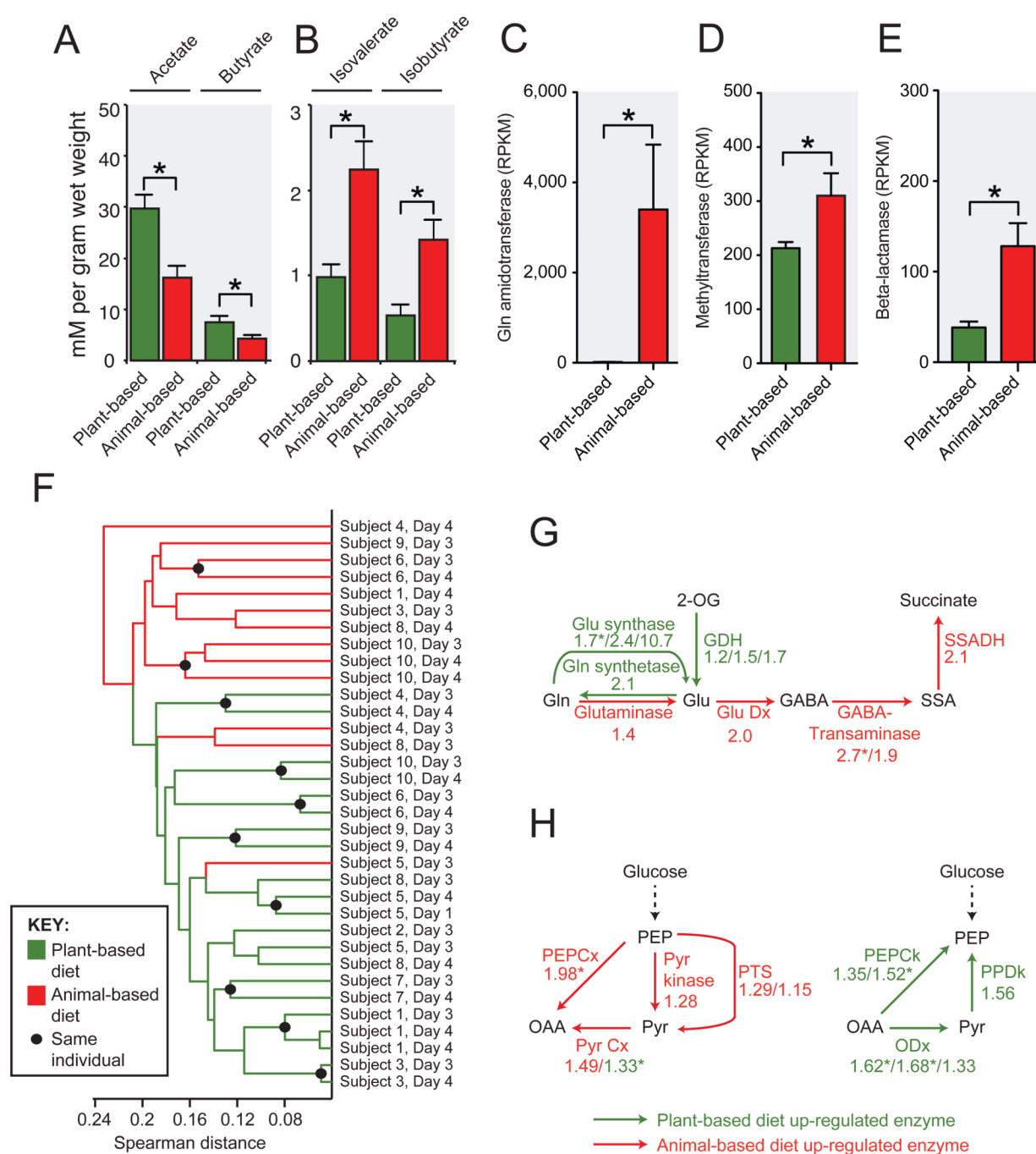
Fig. 3. Diet alters microbial activity and gene expression
