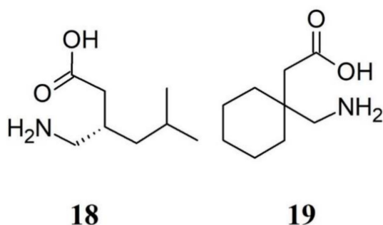
Figure 5. Structure formulae of some gabapentinoids. Numbers correspond to molecules cited in the text.
