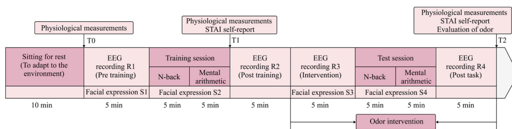
Fig. 1. Experiment procedure.
